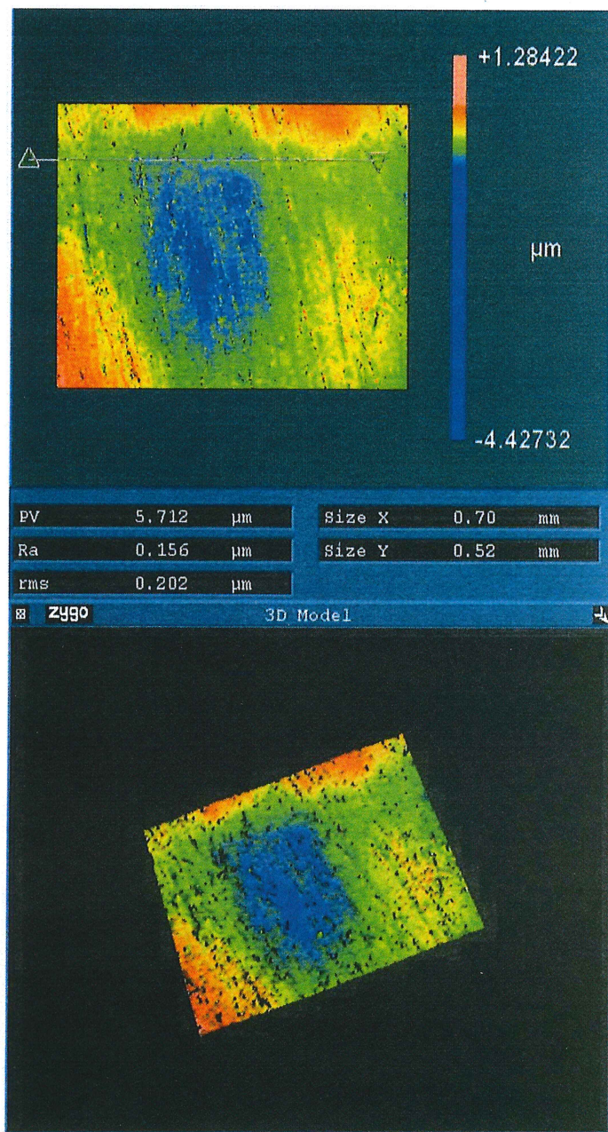
Figure 6. (Profile after treatment; Ra=156nm)
